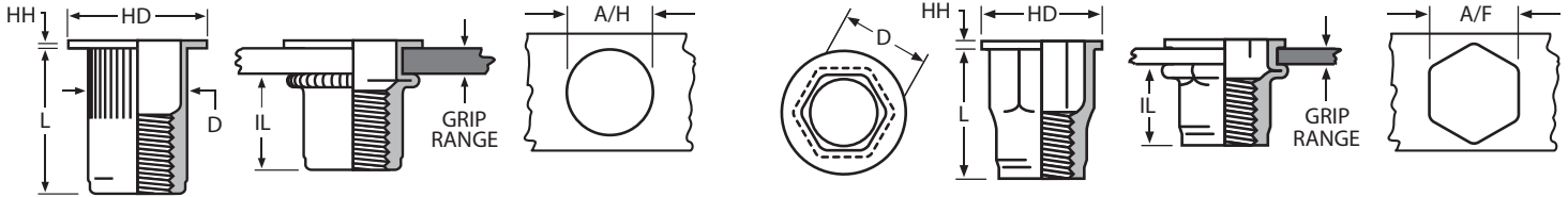
(E-L) OPEN END TYPE
